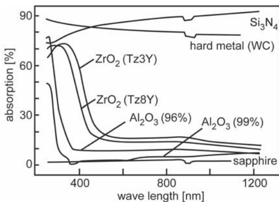
Figure 4.5: The absorption of ceramics depends on wavelength. With the option of efficient nonlinear frequency conversion to 532 nm, 355 nm and 266 nm laser characteristics and material properties like wavelength dependent absorption can be matched.
